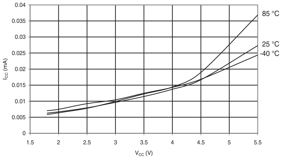
Figure 31-197. ATmega168A: Idle Supply Current vs. V_{CC} (Internal RC Oscillator, 128kHz)
