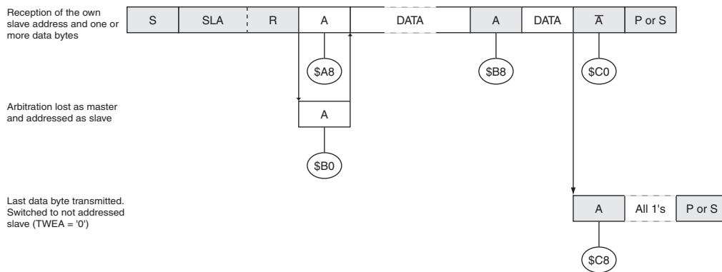
Figure 22-18. Formats and States in the Slave Transmitter Mode
